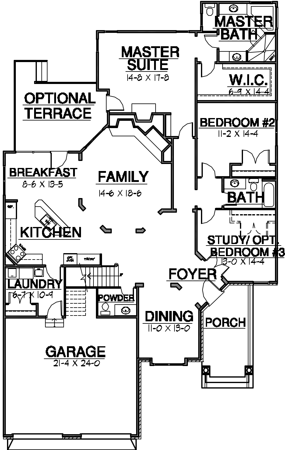
Floor Plan
